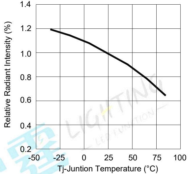
Fig.6-Relative Radiant Intensity vs. Junction Temperature
