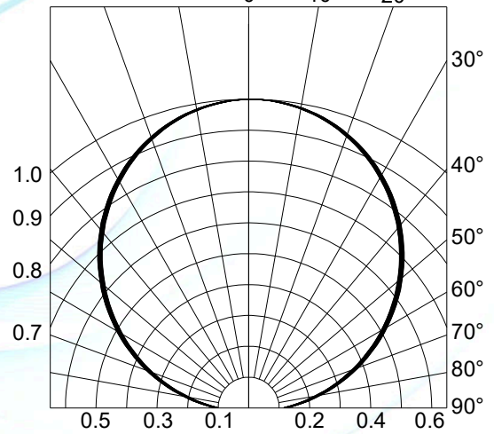
Fig.4-Radiation Diagram T_a=25^\circ\text{C}
