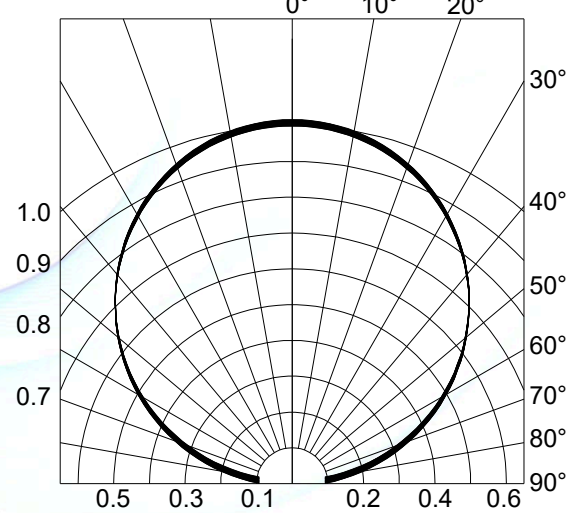
Fig.4-Radiation Diagram T_a=25^\circ\text{C}
