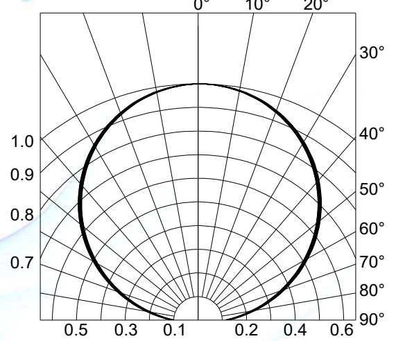
Fig.4-Radiation Diagram T_a=25^\circ\text{C}
