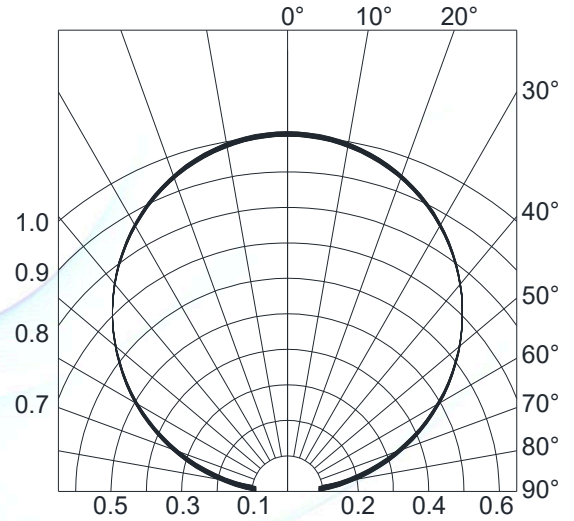
Fig.4-Radiation Diagram
