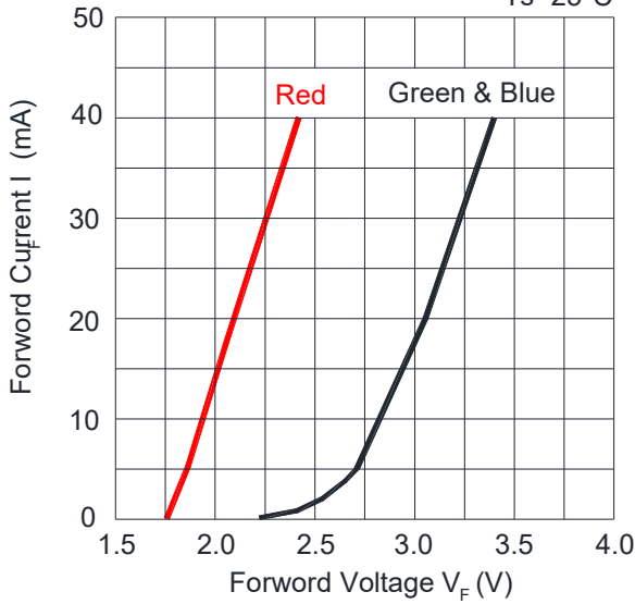
Fig.1-Forward Current(V) vs.
