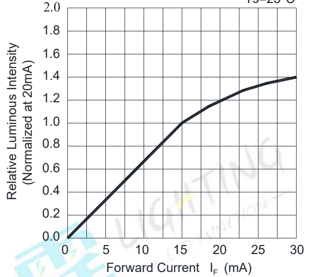
Fig.2-Relative Luminous Intensity
