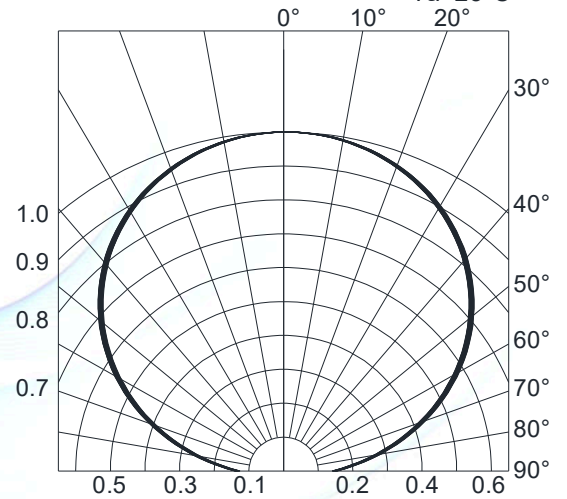
Fig.4-Radiation Diagram T_a=25^{\circ}\text{C}
