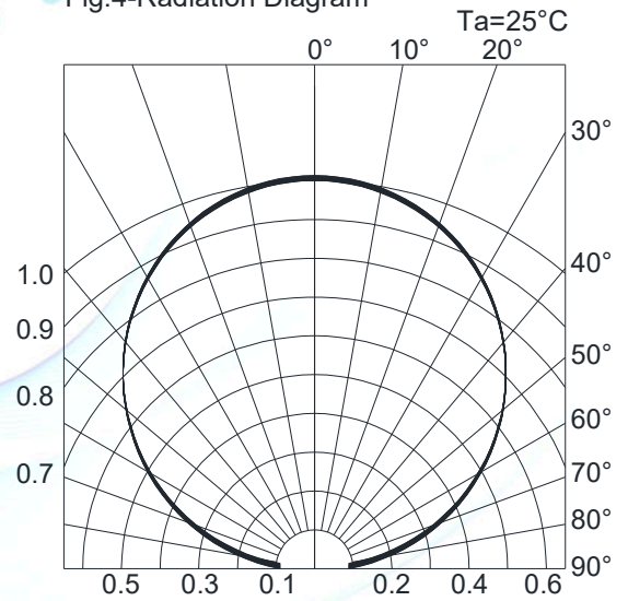
Fig.4-Radiation Diagram T_a=25^\circ\text{C}
