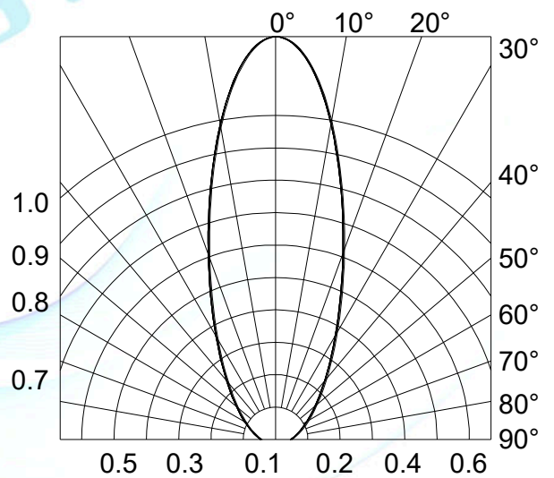
Fig.4-Radiation Diagram T_a=25^\circ\text{C}
