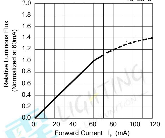
Fig.2-Relative Luminous Flux vs. Forward Current T_s=25^\circ\text{C}
