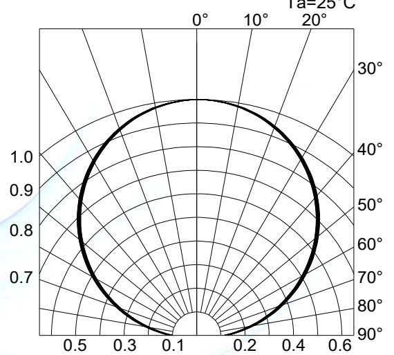
Fig.4-Radiation Diagram T_a=25^\circ\text{C}
