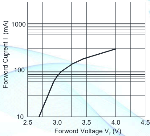
Fig.1-Forward Current(I) vs. Forward Voltage T_s=25^\circ\text{C}
