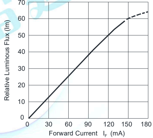
Fig.2-Relative Luminous Flux vs. Forward Current T_s=25^\circ\text{C}
