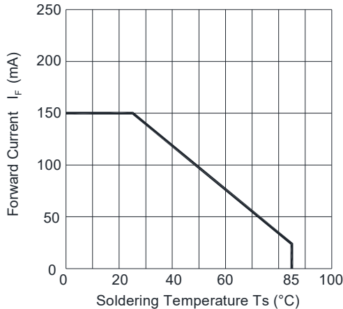
Fig.3-Max. Driving Forward Current vs. Soldering Temperature
