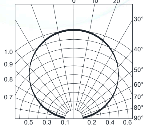
Fig.4-Radiation Diagram T_a=25^\circ\text{C}
