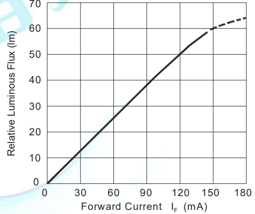
Fig.2-Relative Luminous Flux vs. Forward Current T_s=25^\circ\text{C}
