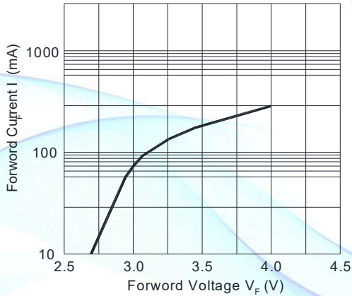
Fig.1-Forward Current(I) vs. Forward Voltage T_s=25^\circ\text{C}
