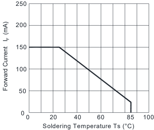
Fig.3-Max. Driving Forward Current vs. Soldering Temperature
