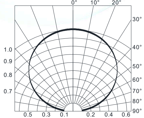
Fig.4-Radiation Diagram T_a=25^\circ\text{C}
