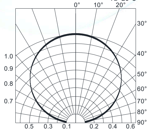
Fig.4-Radiation Diagram T_a=25^\circ\text{C}
