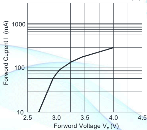
Fig.1-Forward Current (mA) vs. Forward Voltage T_s=25^\circ\text{C}
