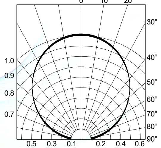
Fig.4-Radiation Diagram T_a=25^\circ\text{C}
