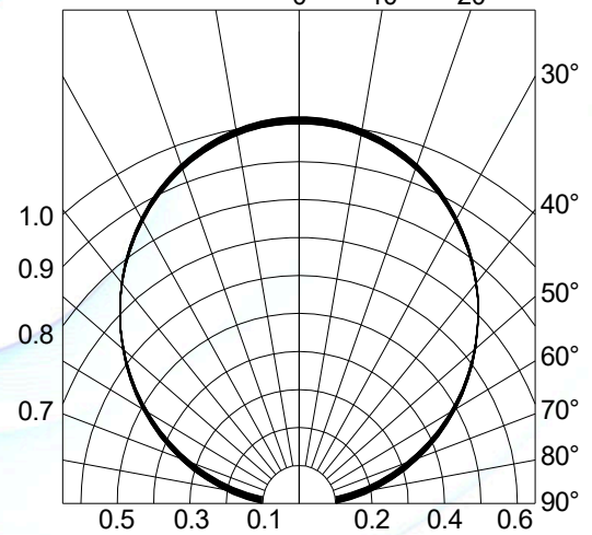
Fig.4-Radiation Diagram T_a=25^\circ\text{C}
