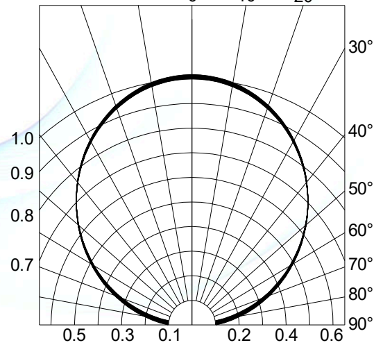
Fig.4-Radiation Diagram T_a=25^\circ\text{C}
