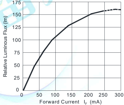
Fig.2-Relative Luminous Flux vs. Forward Current I F (mA) Ts=25°C
