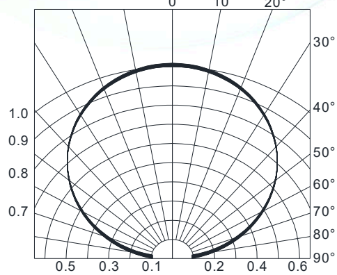
Fig.4-Radiation Diagram Ta=25°C
