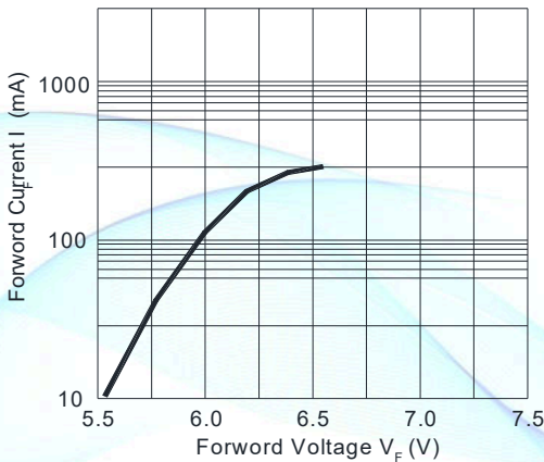
Fig.1-Forward Current(I F ) vs. Forward Voltage V F (V) Ts=25°C
