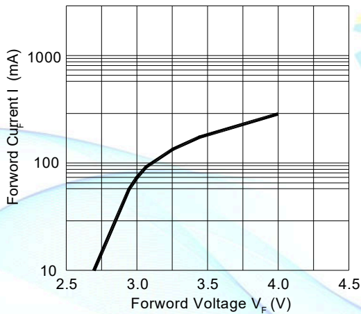
Fig.1-Forward Current(I) vs. Forward Voltage T_s=25\text{ C}
