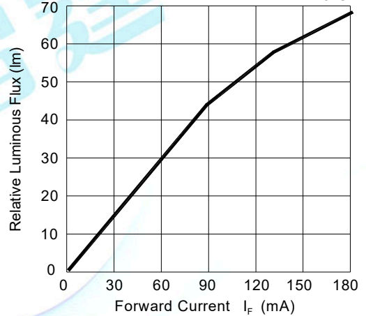
Fig.2-Relative Luminous Flux vs. Forward Current T_s=25\text{ C}
