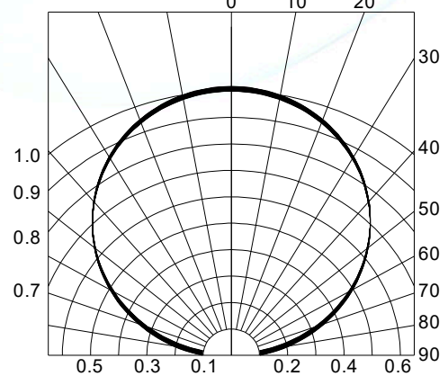
Fig.4-Radiation Diagram T_a=25\text{ C}
