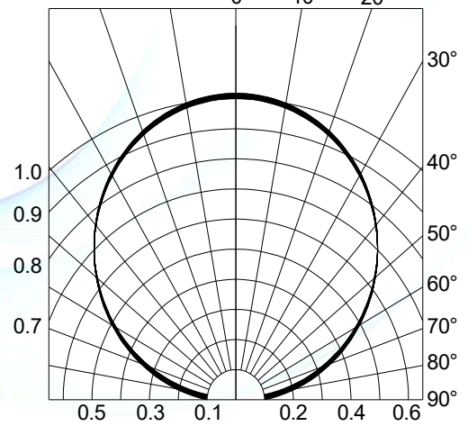
Fig.4-Radiation Diagram T_a=25^\circ\text{C}
