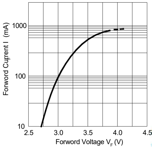
Fig.1-Forward Current(V) vs. Forward Voltage T_s=25^\circ\text{C}
