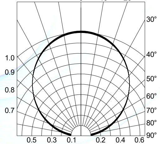
Fig.4-Radiation Diagram T_a=25^\circ\text{C}
