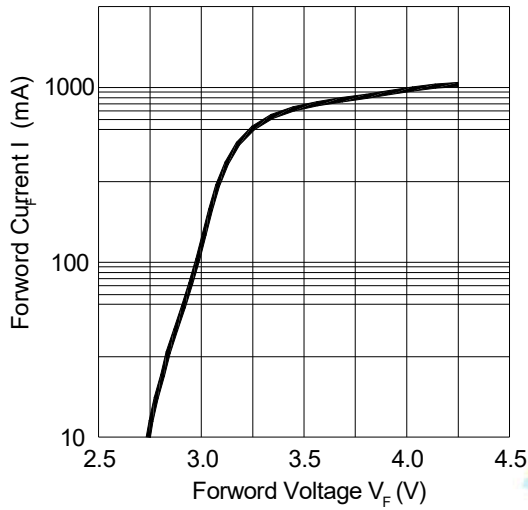
Fig.1-Forward Current(I) vs. Forward Voltage T_s=25^\circ\text{C}
