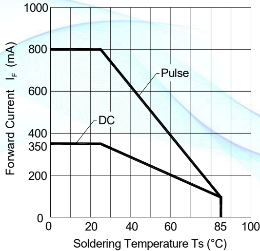
Fig.3-Max. Driving Forward Current vs. Soldering Temperature
