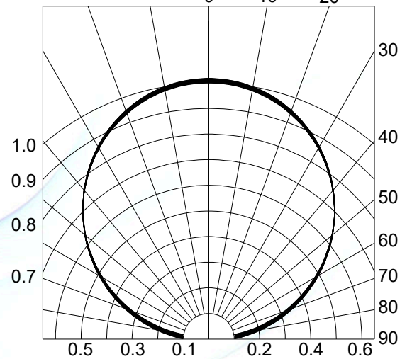
Fig.4-Radiation Diagram T_a=25\text{ C}
