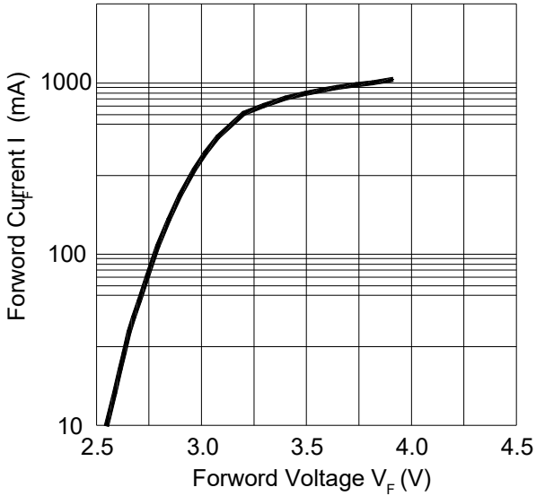
Fig.1-Forward Current(I) vs. Forward Voltage T_s=25\text{ C}
