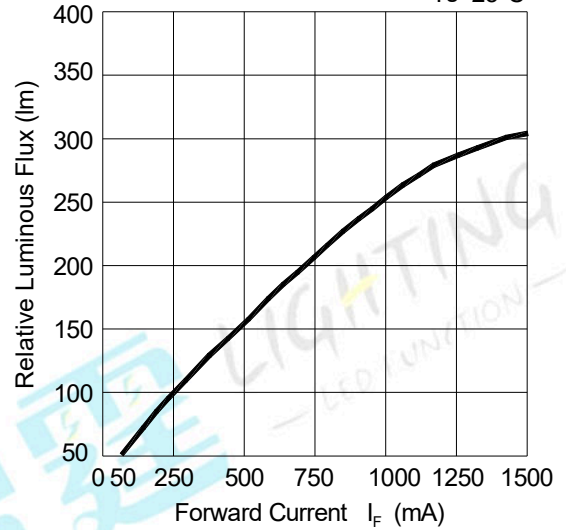
Fig.2-Relative Luminous Flux vs. Forward Current T_s=25^\circ\text{C}
