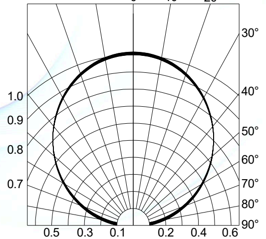
Fig.4-Radiation Diagram T_a=25^\circ\text{C}
