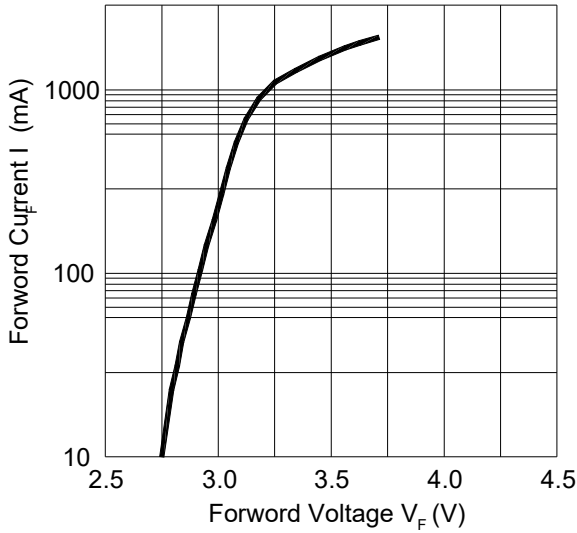
Fig.1-Forward Current(I) vs. Forward Voltage T_s=25\text{ C}
