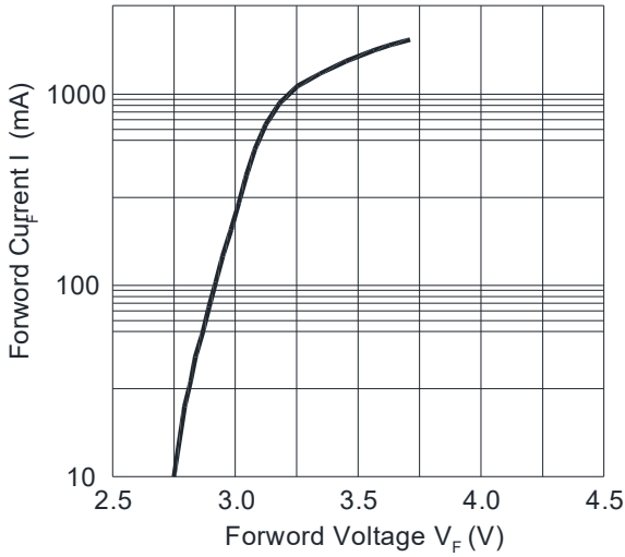
Fig.1-Forward Current(I) vs. Forward Voltage T_s=25^\circ\text{C}
