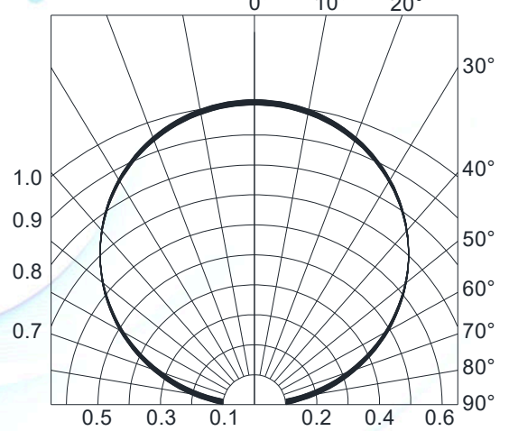
Fig.4-Radiation Diagram T_a=25^\circ\text{C}
