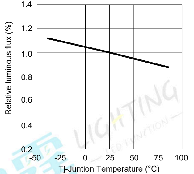
Fig.6-Relative Luminous Flux vs. Junction Temperature
