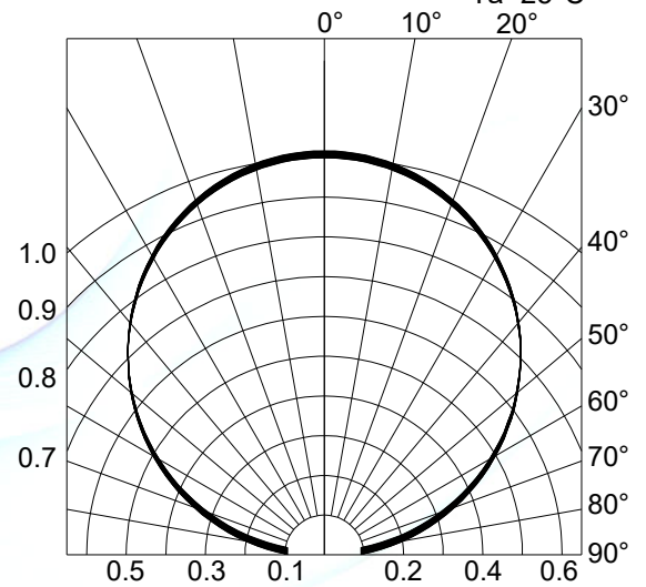
Fig.4-Radiation Diagram T_a=25^{\circ}\text{C}
