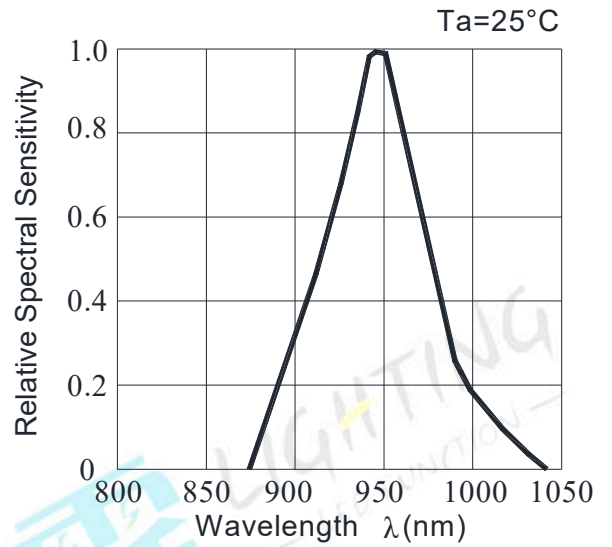
Fig.6-Spectral Sensitivity
