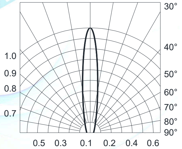
Fig.4-Radiation Diagram T_a=25^\circ\text{C}
