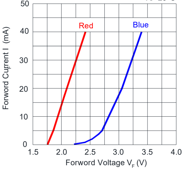
Fig.1-Forward Current(I) vs. Forward Voltage T_s=25^\circ\text{C}
