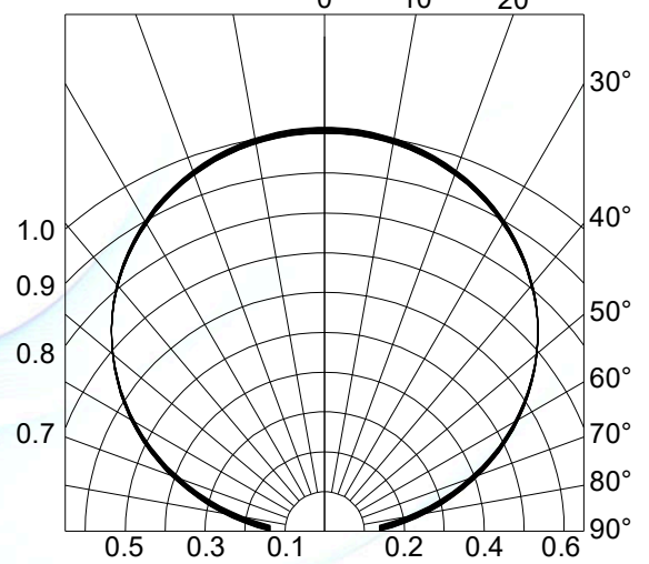
Fig.4-Radiation Diagram T_a=25^\circ\text{C}
