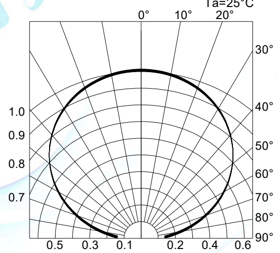
Fig.4-Radiation Diagram T_a=25^{\circ}\text{C}
