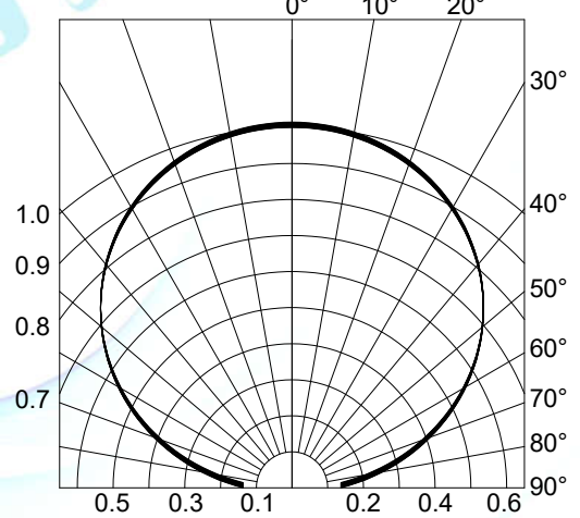
Fig.4-Radiation Diagram T_a=25^{\circ}\text{C}
