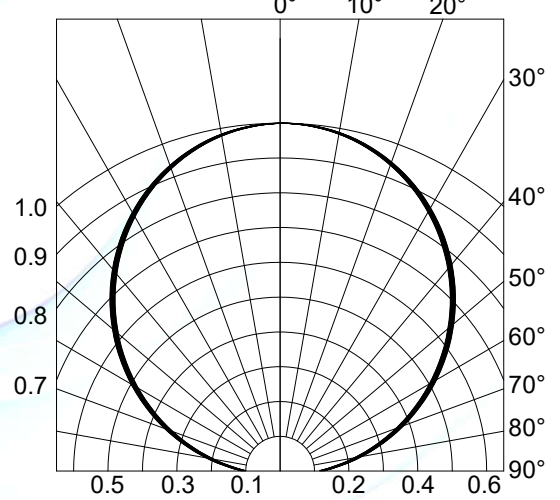
Fig.4-Radiation Diagram T_a=25^\circ\text{C}
