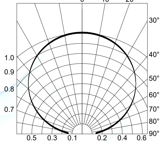
Fig.4-Radiation Diagram T_a=25^\circ\text{C}
