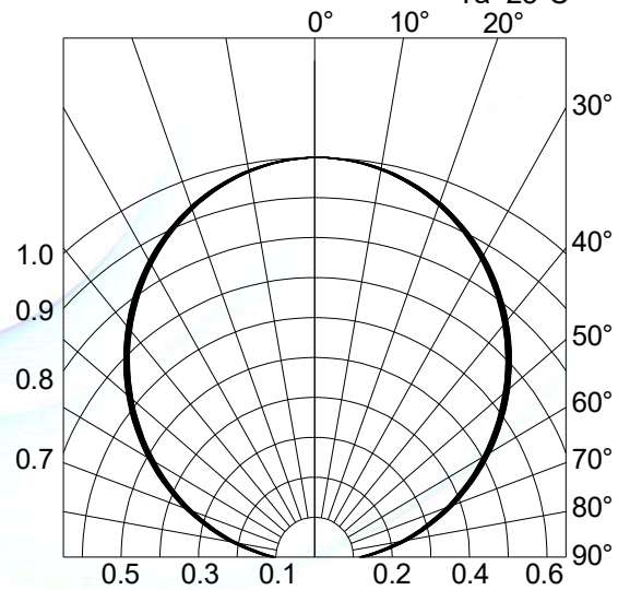
Fig.4-Radiation Diagram T_a=25^\circ\text{C}
