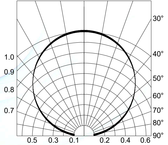
Fig.4-Radiation Diagram T_a=25^\circ\text{C}
