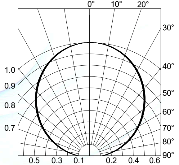
Fig.4-Radiation Diagram T_a=25^\circ\text{C}
