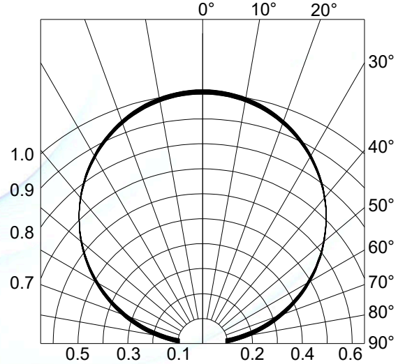
Fig.4-Radiation Diagram T_a=25^\circ\text{C}
