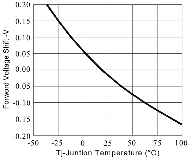
Fig.5-Forward Voltage Shift vs. Junction Temperature
