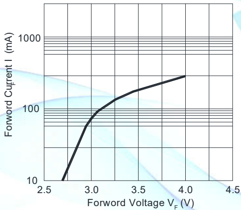
Fig.1-Forward Current(I F ) vs. Forward Voltage (V) T_s=25^{\circ}\text{C}
