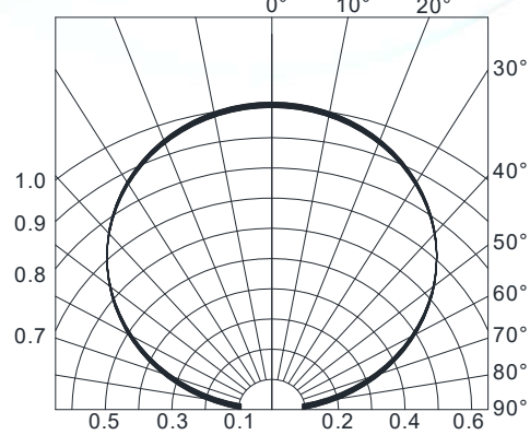
Fig.4-Radiation Diagram T_a=25^\circ\text{C}
