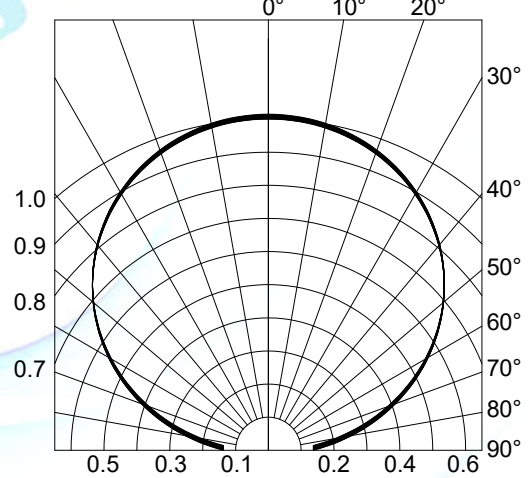
Fig.4-Radiation Diagram T_a=25^{\circ}\text{C}
