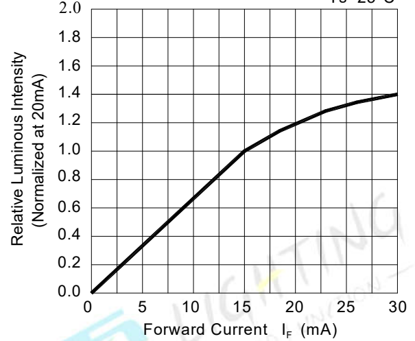
Fig.2-Relative Luminous Intensity vs. Forward Current T_s=25^{\circ}\text{C}
