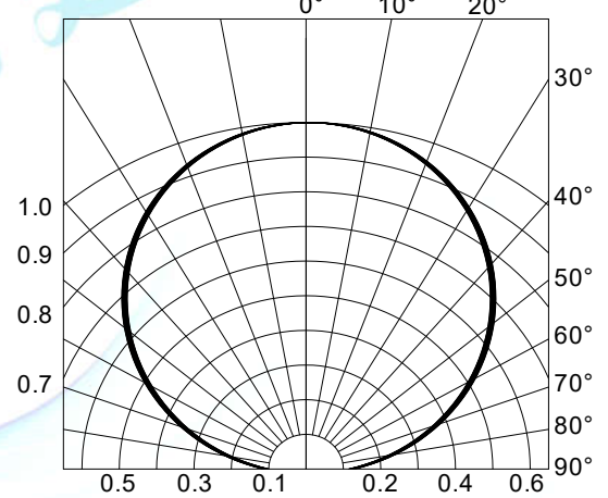
Fig.4-Radiation Diagram T_a=25^{\circ}\text{C}
