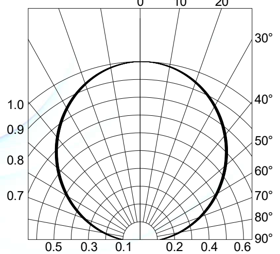
Fig.4-Radiation Diagram T_a=25^{\circ}\text{C}
