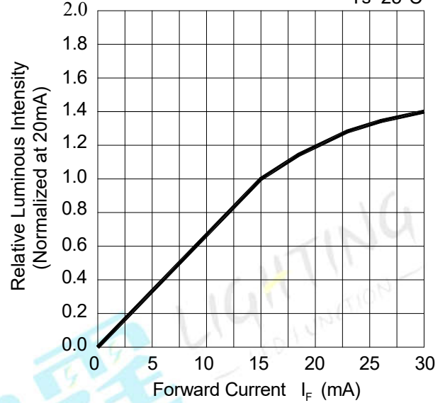
Fig.2-Relative Luminous Intensity vs. Forward Current T_s=25^{\circ}\text{C}
