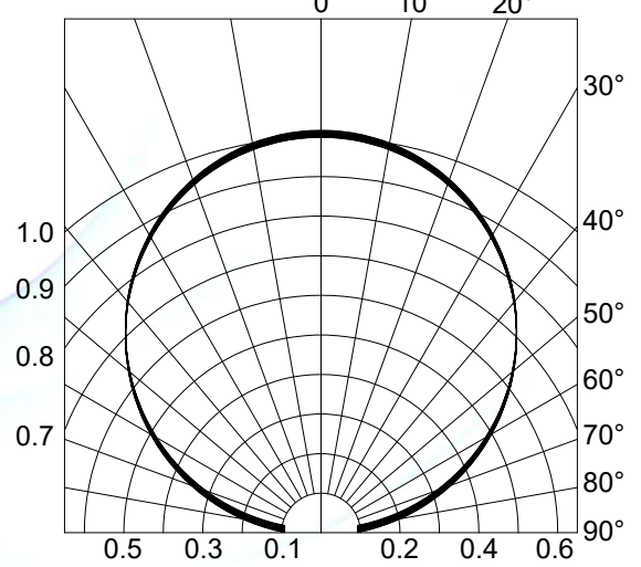
Fig.4-Radiation Diagram T_a=25^{\circ}\text{C}
