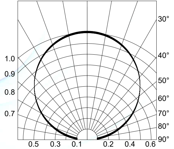
Fig.4-Radiation Diagram T_a=25^\circ\text{C}
