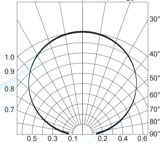
Fig.4-Radiation Diagram T_a=25^\circ\text{C}
