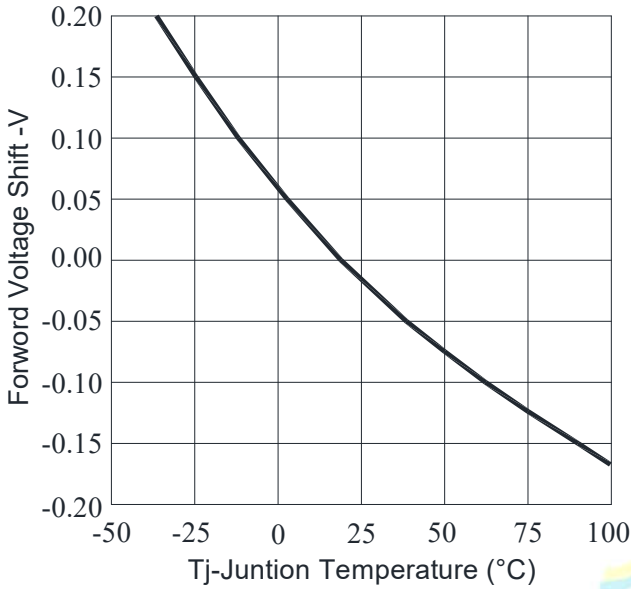
Fig.5-Forward Voltage Shift vs. Junction Temperature
