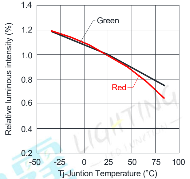
Fig.6-Relative Luminous Intensity vs. Junction Temperature
