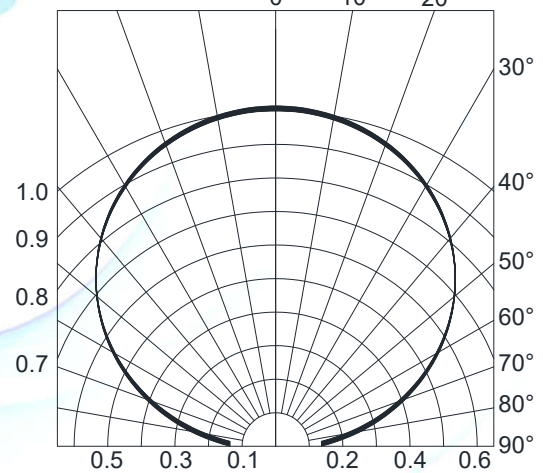
Fig.4-Radiation Diagram T_a=25^{\circ}\text{C}
