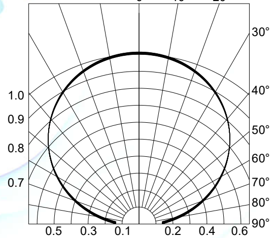
Fig.4-Radiation Diagram T_a=25^{\circ}\text{C}
