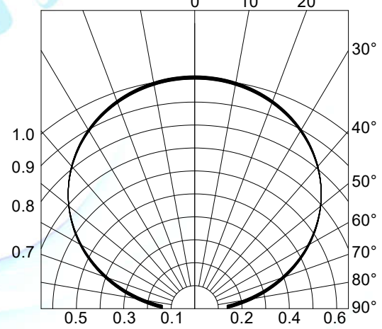
Fig.4-Radiation Diagram T_a=25^\circ\text{C}
