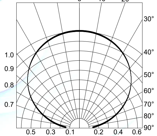
Fig.4-Radiation Diagram T_a=25^\circ\text{C}
