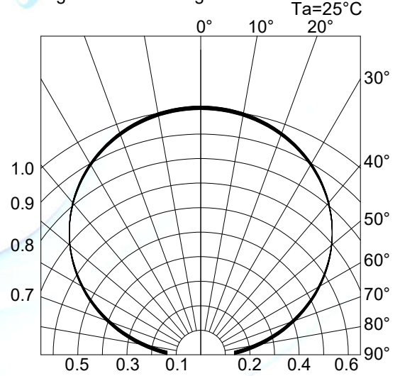
Fig.4-Radiation Diagram T_a=25^\circ\text{C}
