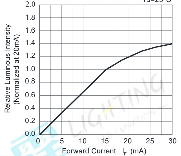
Fig.2-Relative Luminous Intensity vs. Forward Current T_s=25^\circ\text{C}
