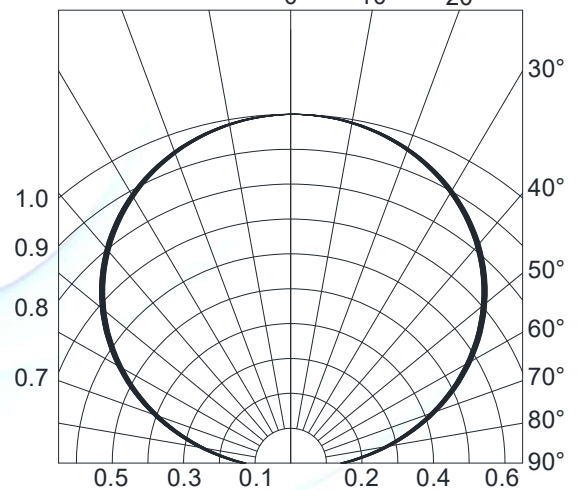
Fig.4-Radiation Diagram T_a=25^\circ\text{C}
